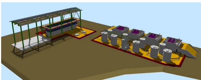
A 3D Model of the Wetar Demonstration Plant
